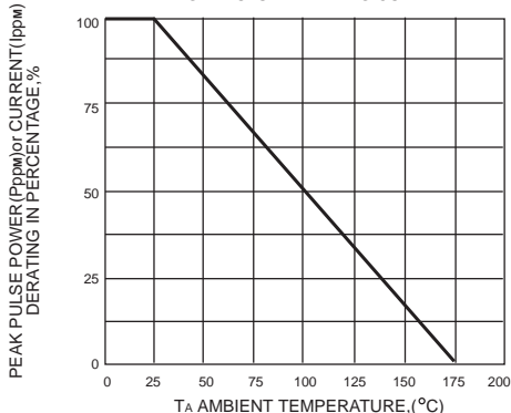
FIG. 2-PULSE DERATING CURVE
